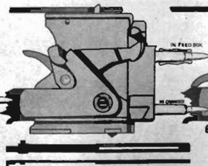
FORWARD READY FOR FIRING
