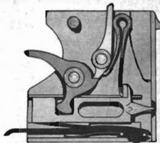
FORWARD READY FOR FIRING
